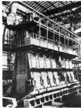
7-cylinders dieselmotor.
