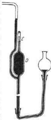
MacLeod-manometer.
